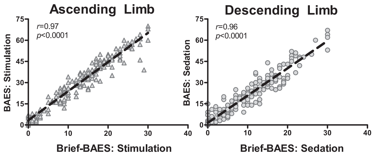
Fig. 1. Correlation between Stimulation ratings measured from the Brief-BAES and the BAES during the rising limb of the BAC (30 minutes after the initiation of beverage consumption), and Sedation ratings during the declining limb of the BAC (120 minutes after the initiation of beverage consumption). Both correlations are from the high alcohol dose (0.8 g/kg).
